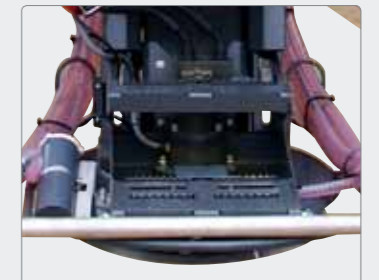
Wide steps integrated in the spreading disc arrangement mean safe and effortless access to the machine house.
